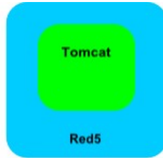
Standalone server
