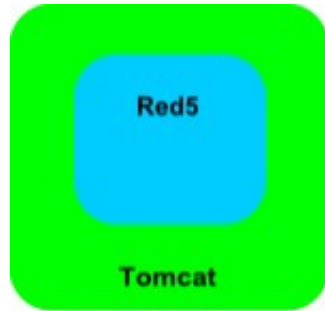
WAR deployment
